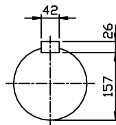
OUTPUT SHAFT
