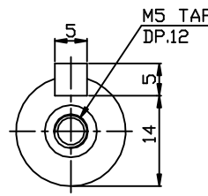
OUTPUT SHAFT
