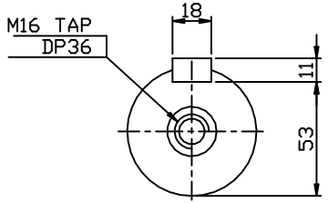
OUTPUT SHAFT
