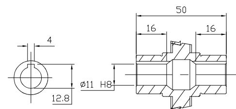
OUTPUT HOLLOW SHAFT
