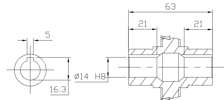
OUTPUT HOLLOW SHAFT
