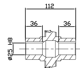
OUTPUT HOLLOW SHAFT
