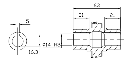
OUTPUT HOLLOW SHAFT
